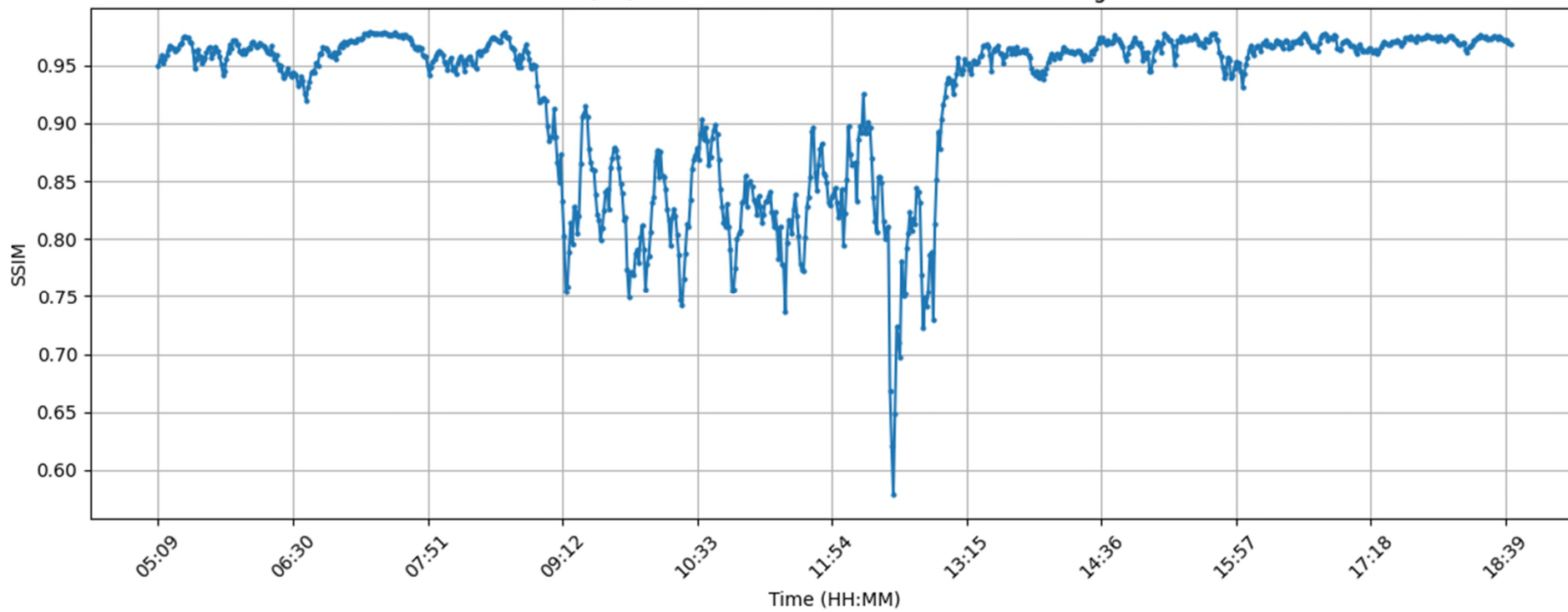
2024/06/14 SSIM between Predicted and True Images
