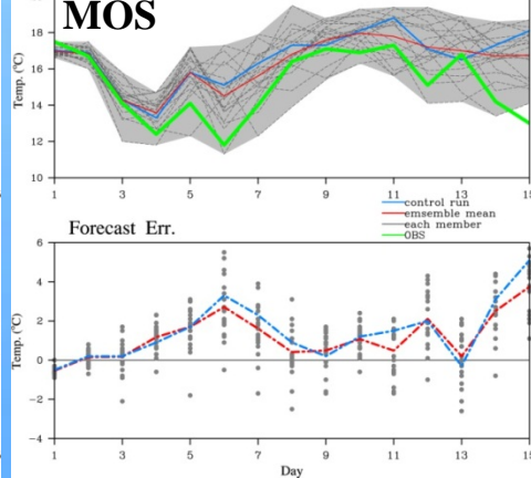
Taipei mos Forecast Verify Initial: 20120119 00Z
