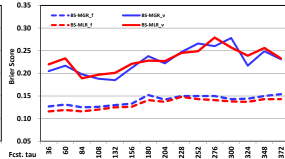
46749 Winter Daily PoP GEFS MGR vs. MLR MOS Brier S
