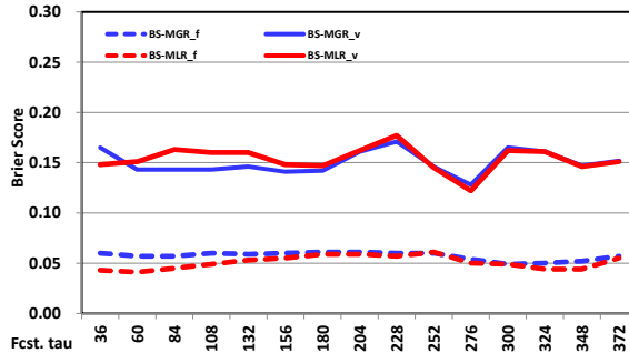
46744 Winter Daily PoP GEFS MGR vs. MLR MOS Brier S
