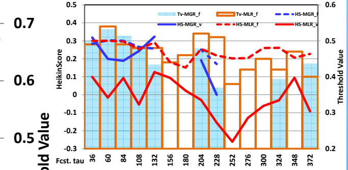
46755 Winter Daily PoP GEFS MGR vs. MLR MOS
