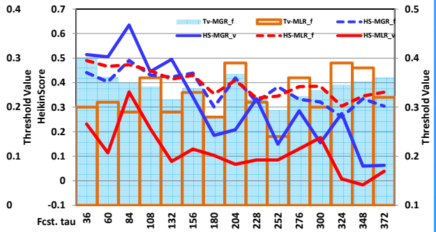
46749 Winter Daily PoP GEFS MGR vs. MLR MOS
