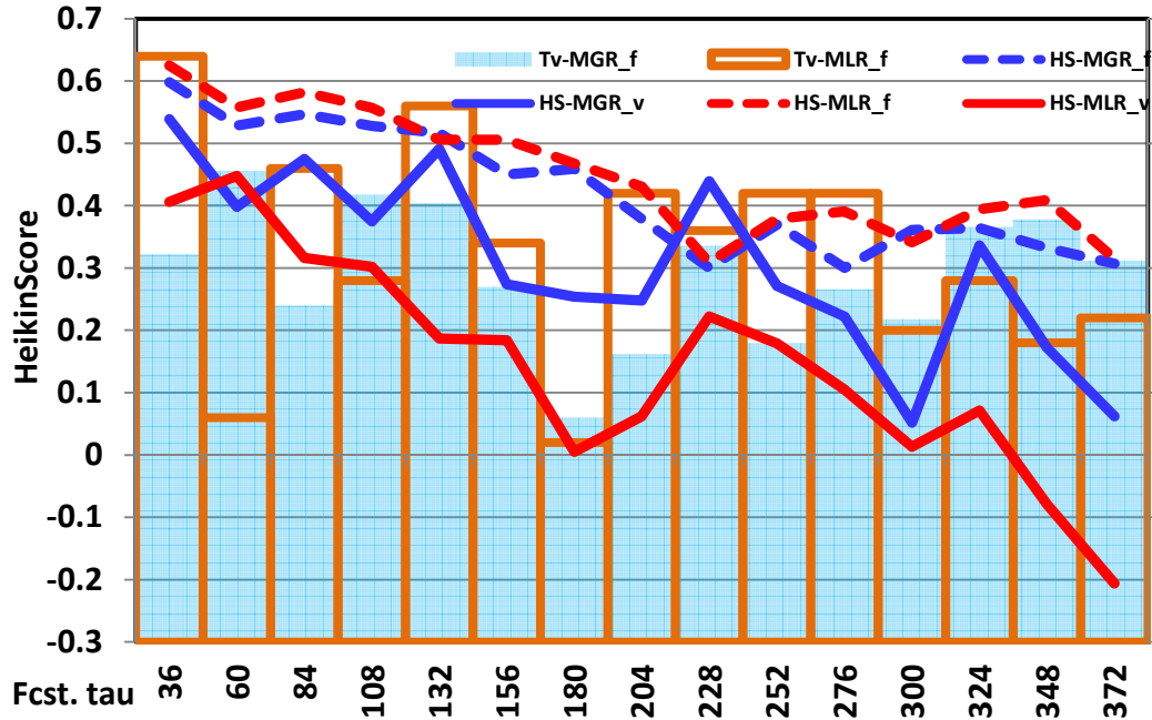
46735 Winter Daily PoP GEFS MGR vs. MLR MOS
