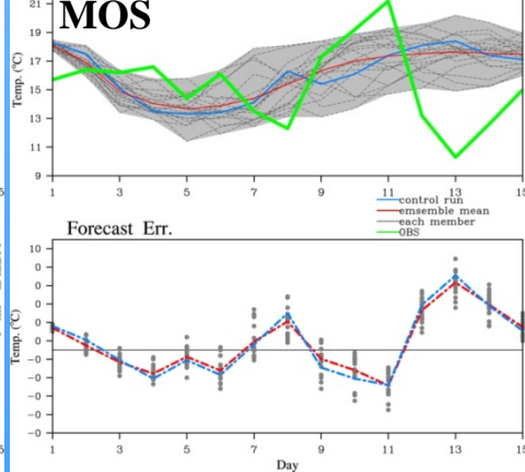
Taipei mos Forecast Verify Initial: 20120126 00Z
