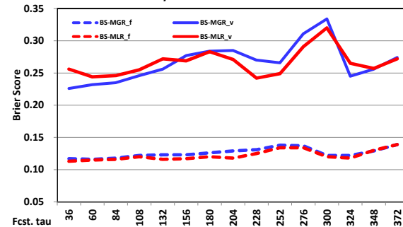
46749 Winter Daily PoP GEFS MGR vs. MLR MOS Brier S
