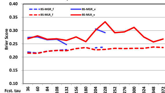
46755 Winter Daily PoP GEFS MGR vs. MLR MOS Brier S
