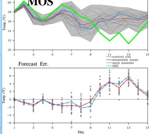
Taipei mos Forecast Verify Initial: 20120112 00Z
