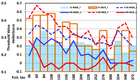
46744 Winter Daily PoP GEFS MGR vs. MLR MOS
