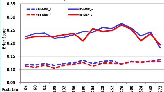
46735 Winter Daily PoP GEFS MGR vs. MLR MOS Brier S
