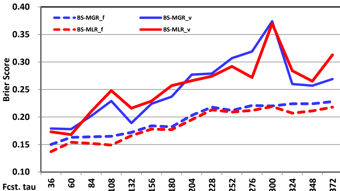
46692 Winter Daily PoP GEFS MGR vs. MLR MOS Brier S
