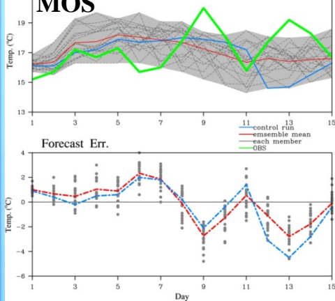
Taipei mos Forecast Verify Initial: 20120105 00Z
